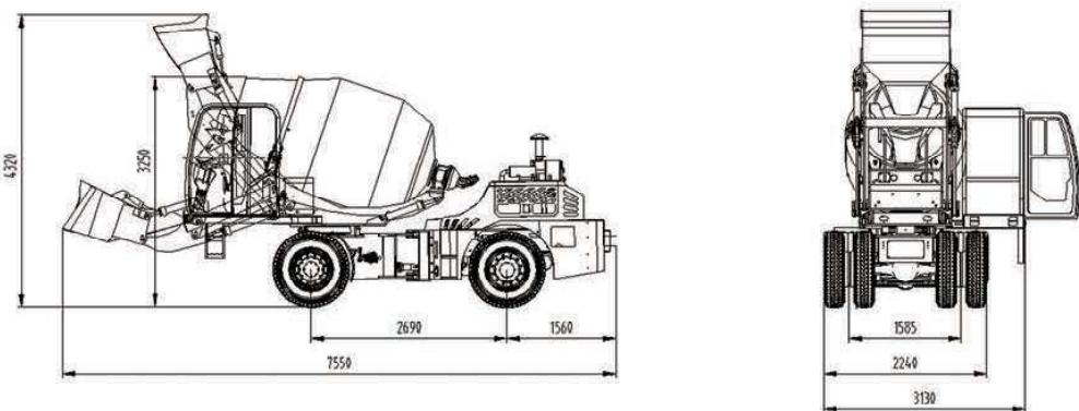
3.5 cubic left front drive self-loading mixer
