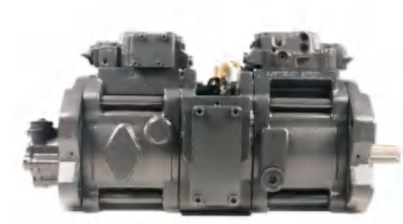
K3V112DTP-9N24-12T(R225-9T,DX225) K3V112DTP-9N24-14T(LG920E,LG922E)
