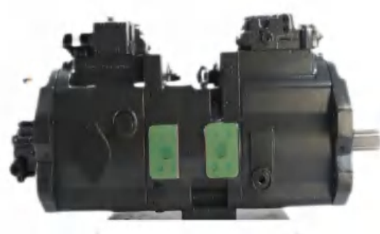
K5V160DTH-9N4A-17T( XG37)
